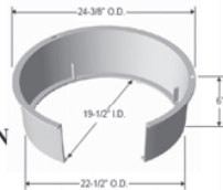
METER BOX EXTENSION
