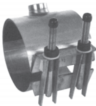
3412AS ALL STAINLESS SADDLE
